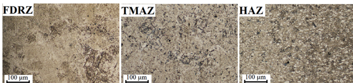
Fig. 8. Optical microstructure of the TiAl6V4 weld joint.
